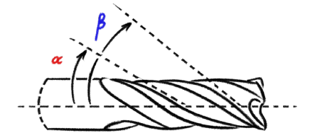
Variable helix angle
