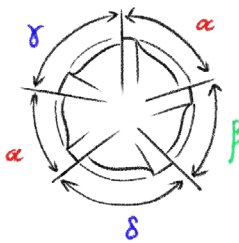
Unequal angular teeth division
