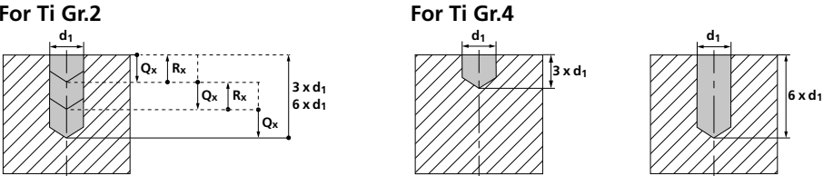
Chip breaking cycle (e.g.: G73)
